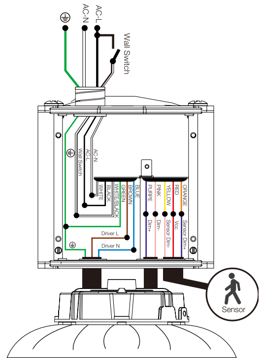
w/DC Sensor SENSOR-ANT-6-4T
