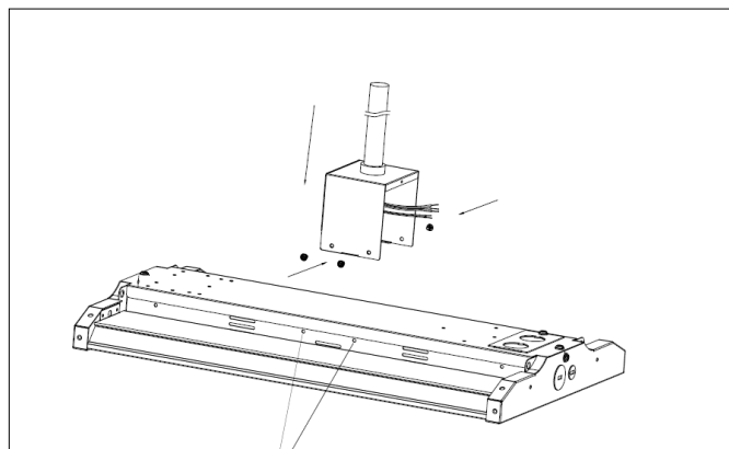
2. Secure the fixture to the pendant mount brackets with 4 screws.
