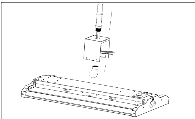
1. Install the pendant mount brackets on the pipe adapter.
