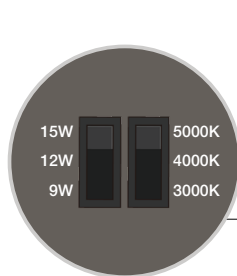
DIP Switch for CCT and Wattage
