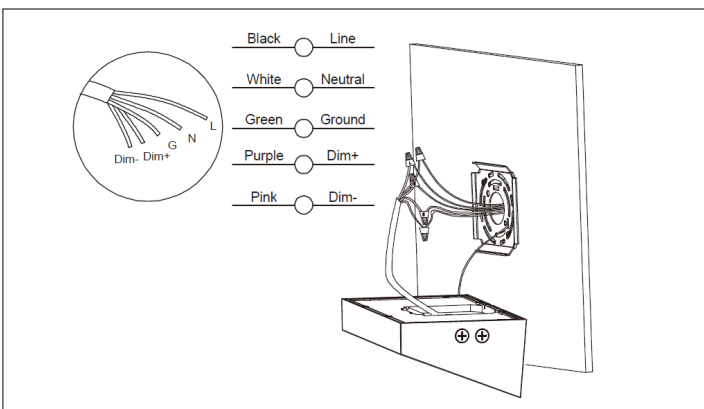
5. Make the wiring connection, according to the wiring diagram. Ensure Power is OFF prior to connecting wiring. CAUTION: Do not pinch wire
