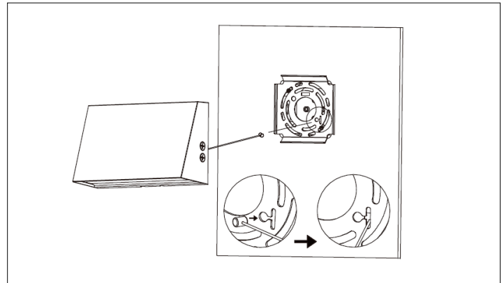
4. Attach the fixture safety cable to the mounting plate on the wall.
