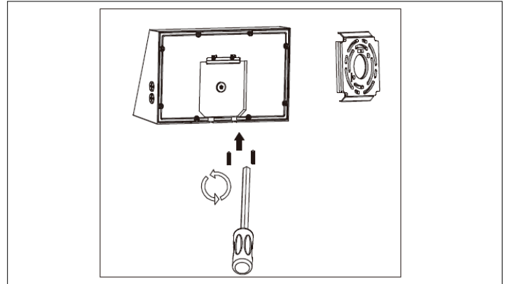
2. Use hex screw driver to remove the mounting plate from the fixture.
