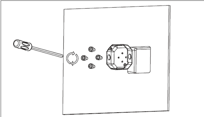
1. Install standard junction box (by others) on the wall.
