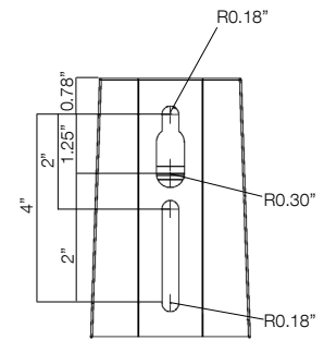
Bracket
