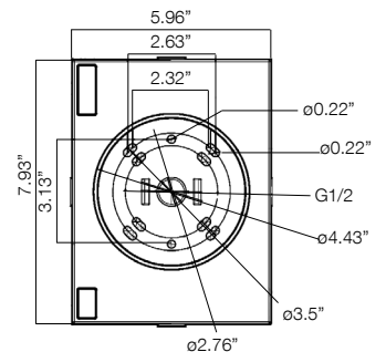
Bracket
