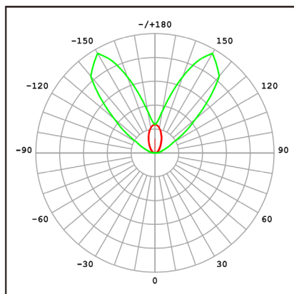
SPN-600 Symmetrical 33° (Dual Module Tilt @ 30°)
