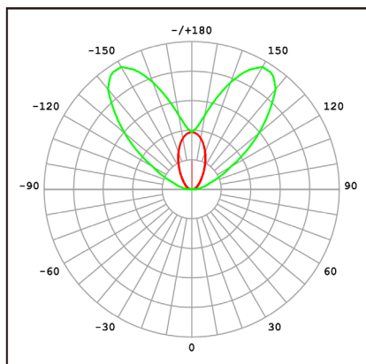
SPN-600 Symmetrical 43° (Dual Module Tilt @ 30°)
