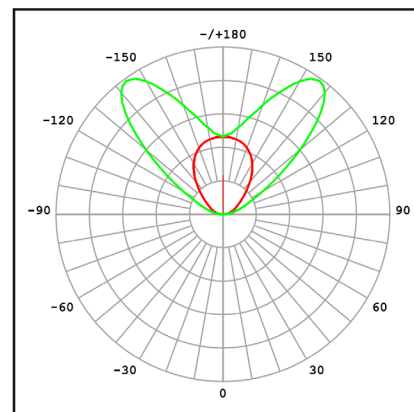
SPN-600 Asymetrical Intense 35°
