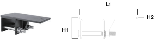
MOUNT-SPM-SBM
