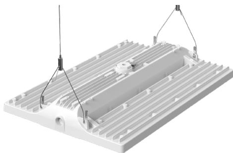
CK 5FT Adjustable aircraft cable hanging kit (standard)
