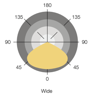
120° 120° Wide Beam Angle (Glass Lens)
