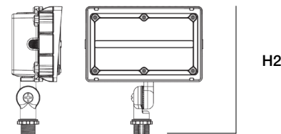
15 / 27W 45 / 60W Knuckle Mount
